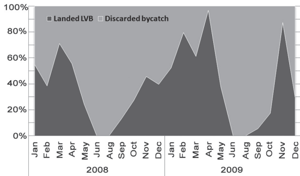
Fig. 6. Monthly trend of LVB (trash) discard ratio from MDT in Mangalore
