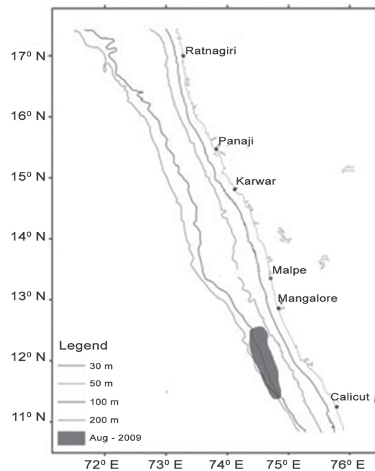
Fig. 8. Fishing ground and month from which highest quantity of discarded fishes from MDT was observed
