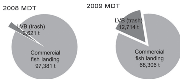
Fig. 4. Landings of commercial fishes and low valued bycatch (trash) by SDT
