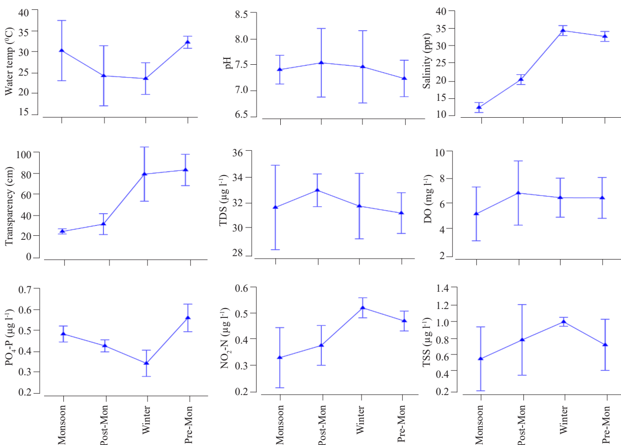
Fig. 2. Variation in nine environmental parameters during the study period in Kohelia Channel, in the northern continental shelf of Bengal Bay, Bangladesh (Post-Mon = Post-monsoon; Pre-mon = Pre-monsoon)
