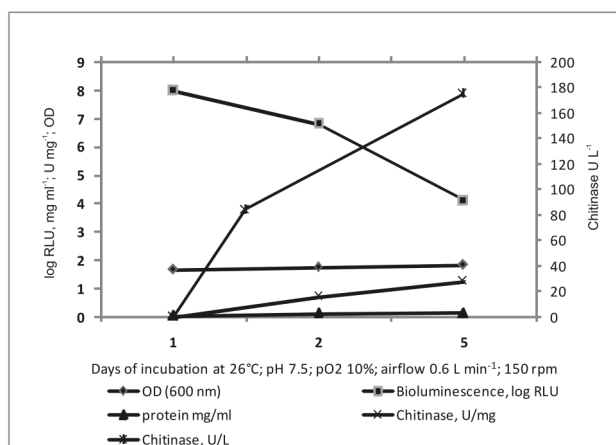
Fig. 3. Production of chitinase by Vibrio harveyi in 2L Biostat® A plus bioreactor
