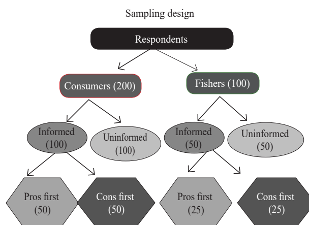
Fig.1. Sampling design
