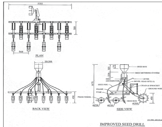
Fig. 1. A view of the improved traditional seed drill.
