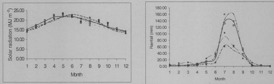
Fig. 1. Observed (symbols) and generated (lines) mean daily radiation (a) and mean monthly rainfall (b) for Pali (○, ----), Jodhpur (□, —), Bikaner (◆, ---) and Jaisalmer (▲, - - -).
