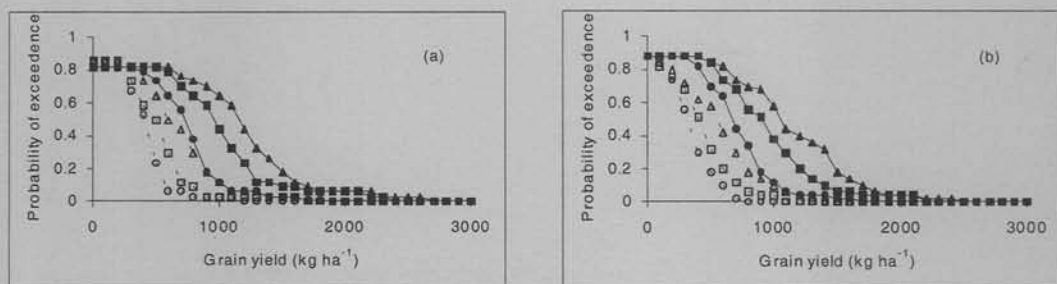
Fig. 4. Probability of exceedence for grain yield simulated over 34 years with observed weather data for Jodhpur (a) and with over 50 years of synthetic weather data (b) for cv. WRajPop (●), HHB67 (■) and RCB-IC911 (▲) without (open symbols) and with (closed symbols) applied nitrogen at 20 kg N ha -1 .
