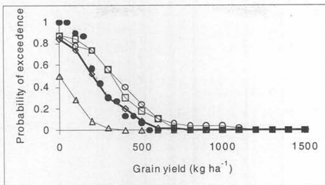
Fig. 2. Probability of exceedence for district grain yield measured over 30 years for Rajasthan (●) compared with the simulated probability for cv. WRajPop without applied nitrogen from Pali (○), Jodhpur (□), Bikaner (△) and Jaisalmer
