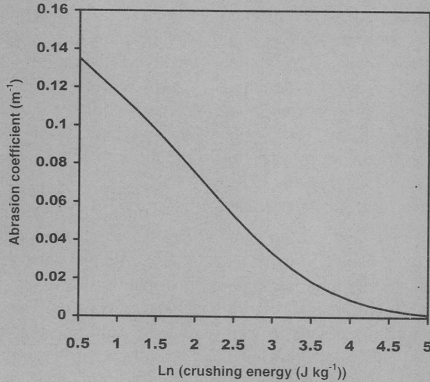
Fig. 2. Abrasion coefficient as a function of dry stability of soil aggregates (Modified from Hagen, et al. , 1992).
