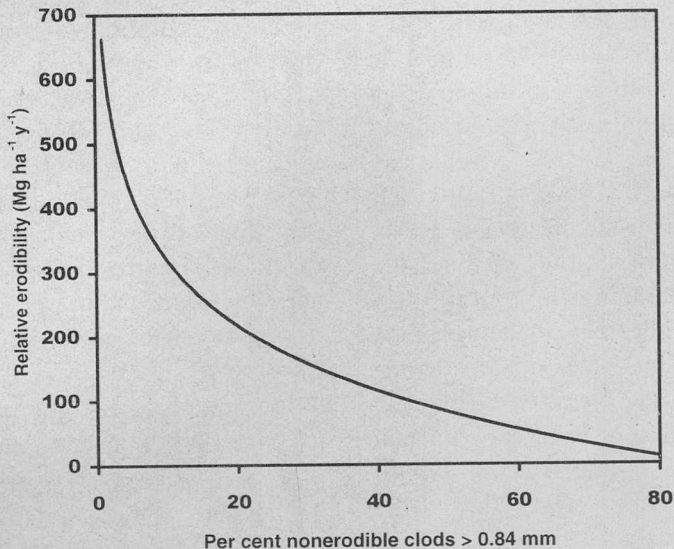
Fig. 1. Relationship between percent nonerodible aggregates > 0.84 mm and relative soil erodibility (Modified from Woodruff and Siddoway, 1965).
