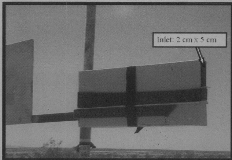
Fig. 1. BSNE airborne sediment sampler.
