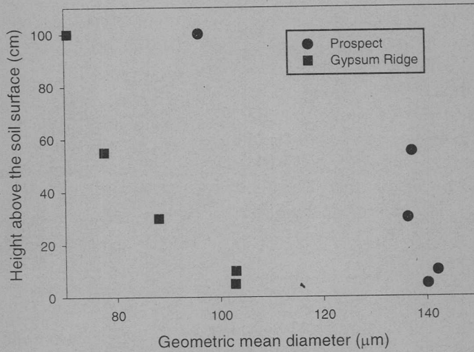
Fig. 10. Geometric mean diameter of airborne sediment at the sites of Prospect and Gypsum Ridge, near Twentynine Palms, California, USA.
