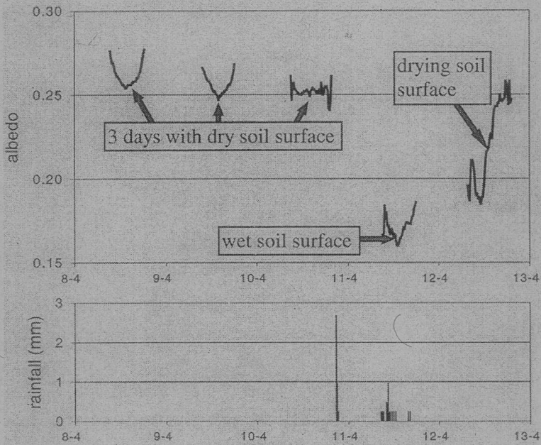
Fig. 12. Albedo and rainfall for 8 April through 12 April, 2001 on a field near Burlington, Colorado, USA. Albedo decreases after rain has wetted the soil surface. It increases again on 12 April, as the soil surface is drying.
