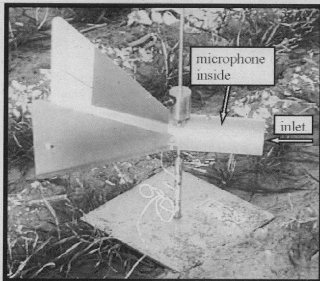
Fig. 6. Saltiphone automated, continuous saltation detector.
