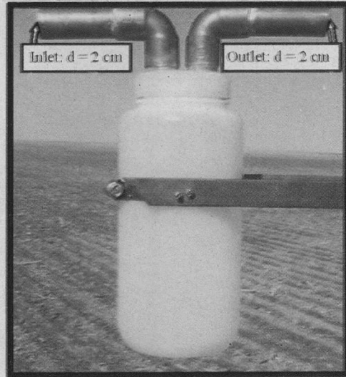
Fig. 2. MWAC airborne sediment sampler. This version was constructed at the Wind Erosion Research Unit in Manhattan, Kansas, USA. It is larger than what most other researchers have used.
