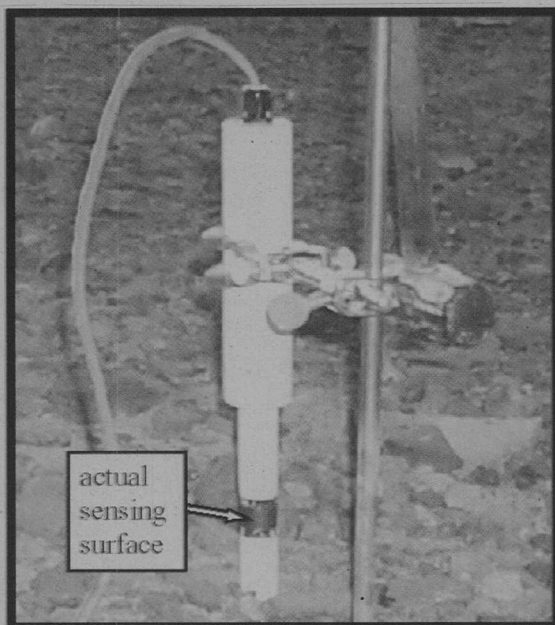
Fig. 5. Sensit automated, continuous saltation detector.
