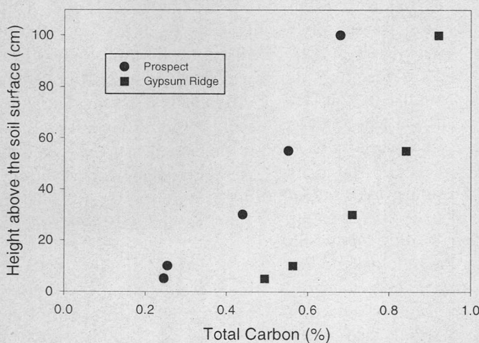
Fig. 11. Carbon concentration of airborne sediment at the sites of Prospect and Gypsum Ridge, near Twentynine Palms, California, USA.
