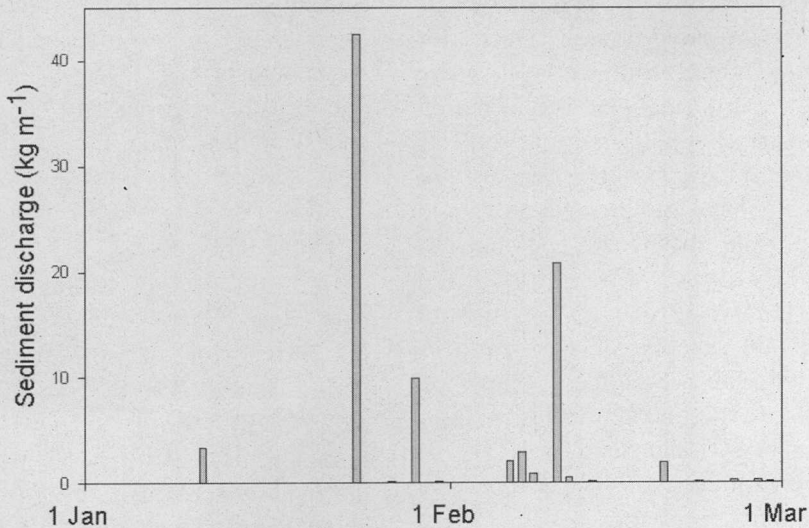
Fig. 9. Daily sediment discharge ( \text{kg m}^{-1} ) on a site near Twentynine Palms, California, USA, based on monthly sediment discharge measured using BSNE samplers and daily Sensit particle count.
