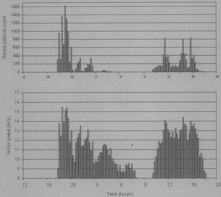
Fig. 7. Wind erosion on a field near Burlington, Colorado, USA on 17 and 18 December, 2000. Wind speed was measured at a height of 2 m. Data are 15 minute averages.
