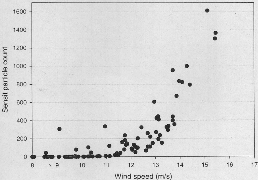
Fig. 8. Determination of threshold wind speed from Sensit and wind speed data. Wind speed was measured at a height of 2 m. Same data as in Fig. 7.
