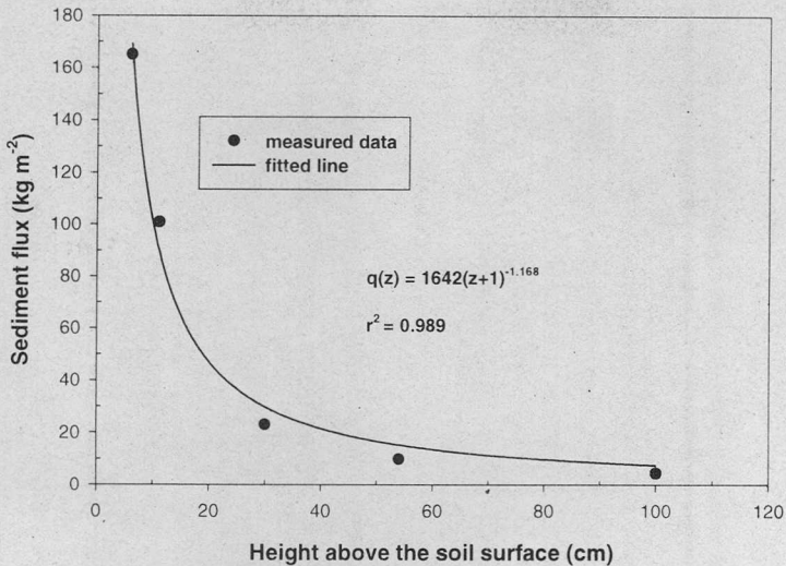
Fig. 4. Sediment flux for January, 2001 on a site near Twentynine Palms, California, USA. The area under the fitted curve represents sediment discharge.
