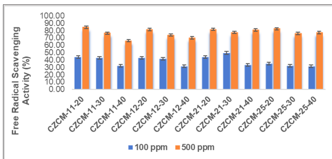
Fig. 3. Free radical scavenging activity of fruits of different genotypes of Cordia myxa (CZCM-11, CZCM-12, CZCM-21, CZCM-25) at different maturity stages i.e. 20, 30 and 40 days after fruit set).
