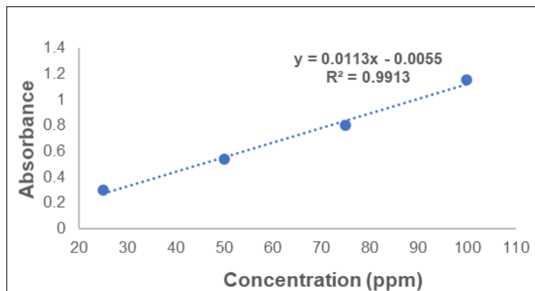
Fig. 2. Standard curve for gallic acid.
