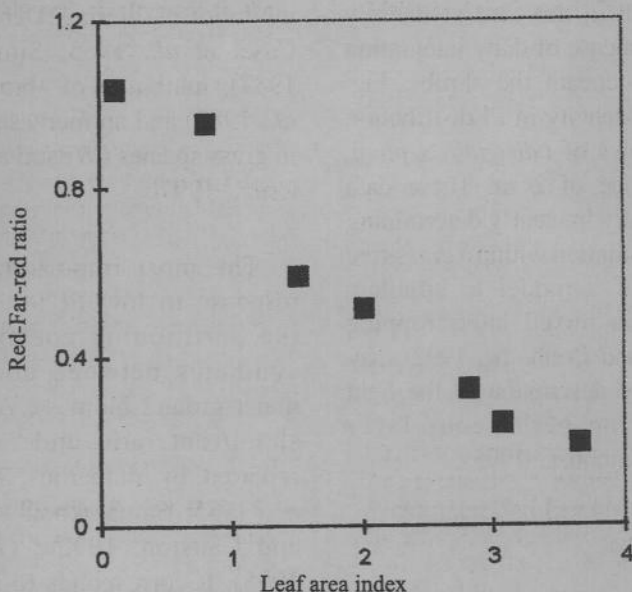
Fig. 2. Relation between red:far red ratio at ground level and leaf area index of the canopy (from Holmes and Smith, 1977).
