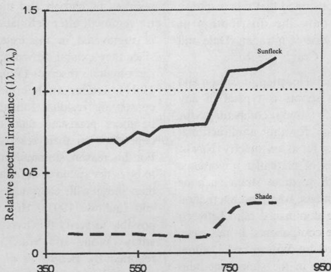
Fig. 1. Special energy distribution of light at ground level ( I_\lambda ) and above the canopy ( I_{\lambda 0} ) (from Varlet-Grancher et al. , 1993).
