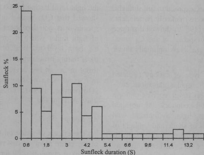
Fig. 7. Daily proportion for the most frequent sunfleck durations between two rows of Gliricidia sepium . Row spacing = 3 m. Global LAI = 1.7 (from Dulormne, 1997).
