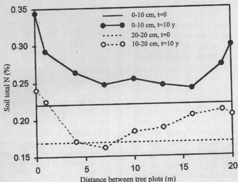
Fig. 10. Concentration of soil nitrogen in a grass plot ( Dichanthium spp.) placed between two silvopastoral plots ( Gliricidia sepium , NFT). The tree rows correspond to distances 0 and 20 m; t = 0 and t = 10 y correspond to nitrogen concentration at the time of tree planting and 10 y afterwards, respectively (adapted from Dulormne et al. , 1999); soil depth sampled: 0-10 cm, 10-20 cm.
