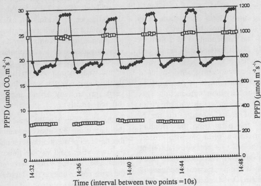
Fig. 9. Net \text{CO}_2 assimilation ( P_n ) of leaves of Digitaria decumbens grown under shade (33% sunlight) exposed alternately to low and high (sunflecks) levels of PPFD (—) (from Dulorme, 1997).
