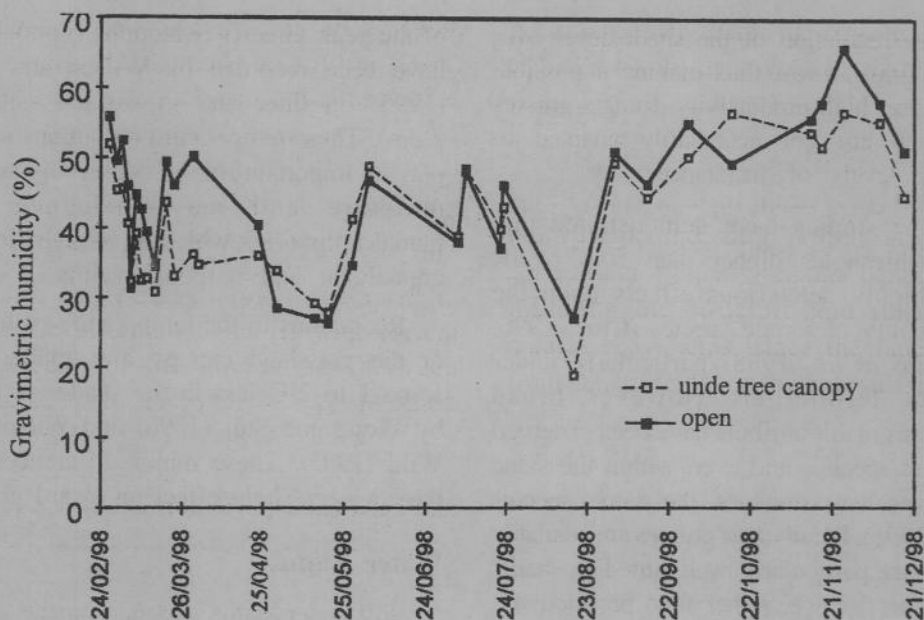
Fig. 4. Annual trend of gravimetric humidity (%) in the top 10 cm of soil under the canopy of Gliricidia sepium and in the open (M. Dulormne and J. Sierra, unpublished data).
