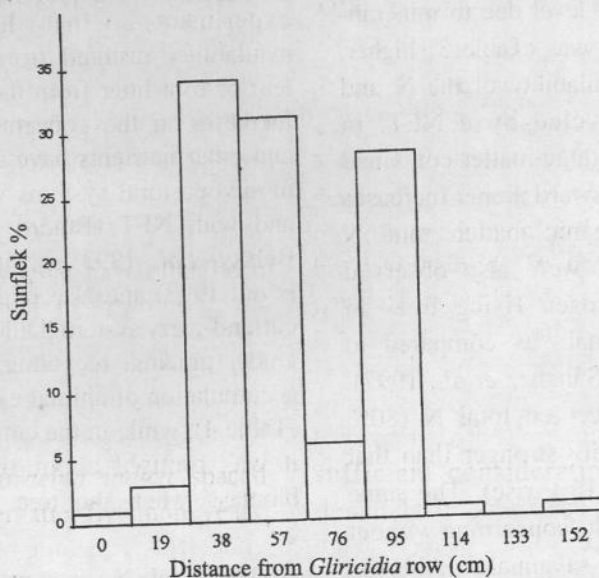
Fig. 8. Spatial distribution of sunflecks between two rows of Gliricidia sepium . Distance between rows = 3 m, IAF = 1.7 (from Dulormne, 1997). Sunfleck = irradiance \geq 800 \mu\text{mol m}^{-2} \text{s}^{-1} for >0.6 s.
