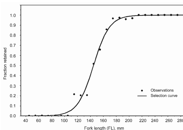
Fig. 1. Selectivity curve in respect of Pampus argenteus
