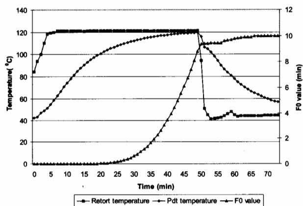
Fig. 2. Heat penetration Characteristics and F_0 value of thermally processed tuna in Oil in a Stationary retort (0 rpm)
