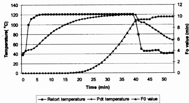
Fig. 8. Heat penetration Characteristics and F_0 value of thermally processed tuna in Oil processed to F_0 value 10 in a rotary retort at 6 rpm
