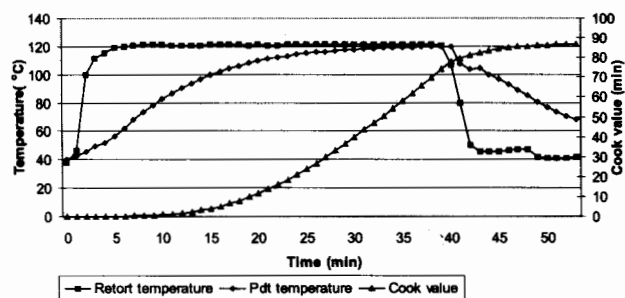
Fig. 9. Heat penetration Characteristics and Cook value of thermally processed tuna in Oil processed to F_0 value 10 in a rotary retort at 6 rpm
