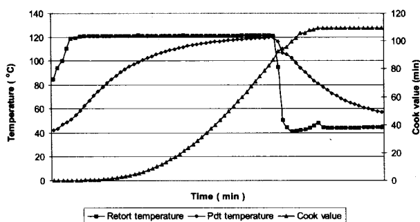
Fig. 3. Heat penetration Characteristics and Cook value of thermally processed tuna in Oil in a Stationary retort (0 rpm)
