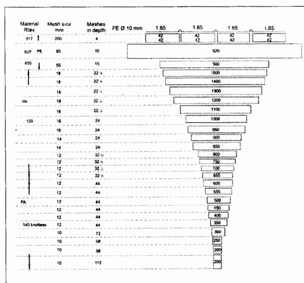
Fig. 2. Design of a typical stake net operated off Vypeen
