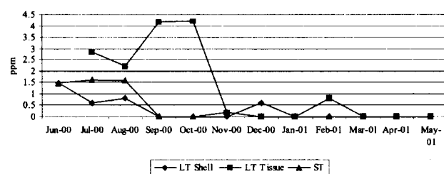
Fig.2. Cadmium concentration (ppm) in short term barnacle, long term barnacle shell and tissues.
