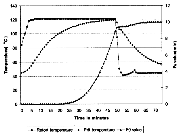
Fig. 4. Heat penetration Characteristics and F_0 value of thermally processed tuna in Oil
