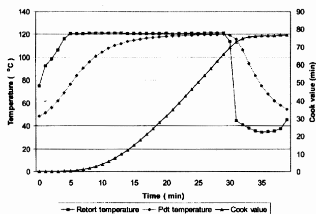
Fig. 5. Heat penetration Characteristics and Cook value of thermally processed tuna in brine
