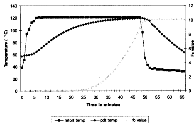
Fig. 3. Heat penetration Characteristics and F_0 value of thermally processed tuna in Tomato sauce
