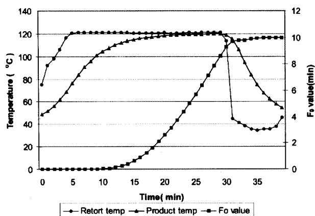
Fig. 1. Heat penetration Characteristics and F_0 value of thermally processed tuna in brine
