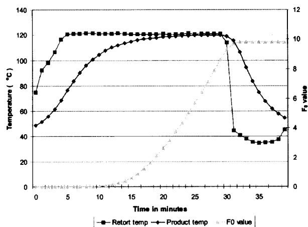
Fig. 2. Heat penetration Characteristics and F_0 value of thermally processed tuna in Curry
