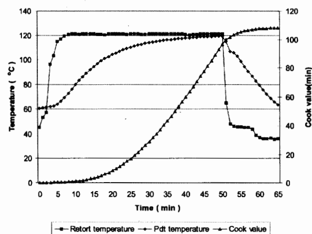
Fig. 6. Heat penetration Characteristics and Cook value of thermally processed tuna in Curry
