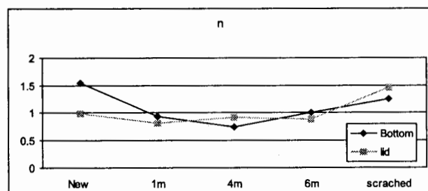
Fig. 1. Constant phase element of TFS can
