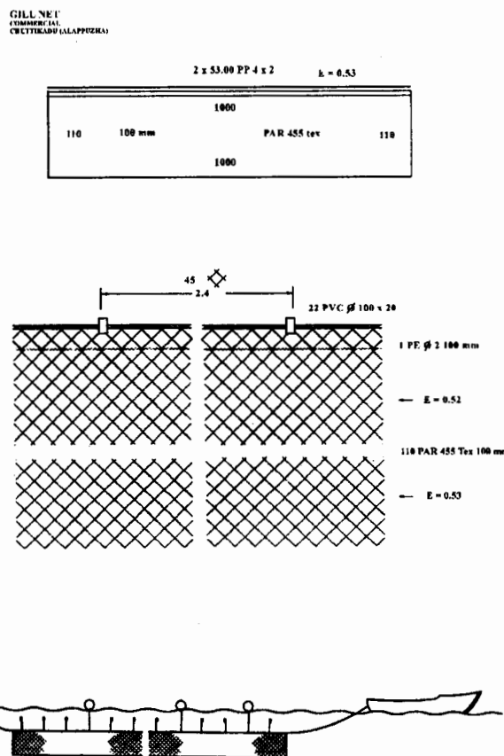
Fig. 2. Design of gill net (PA)
