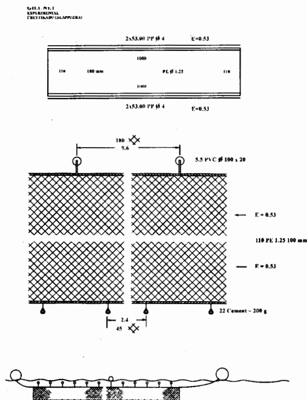
Fig. 1. Design of gill net (PE)
