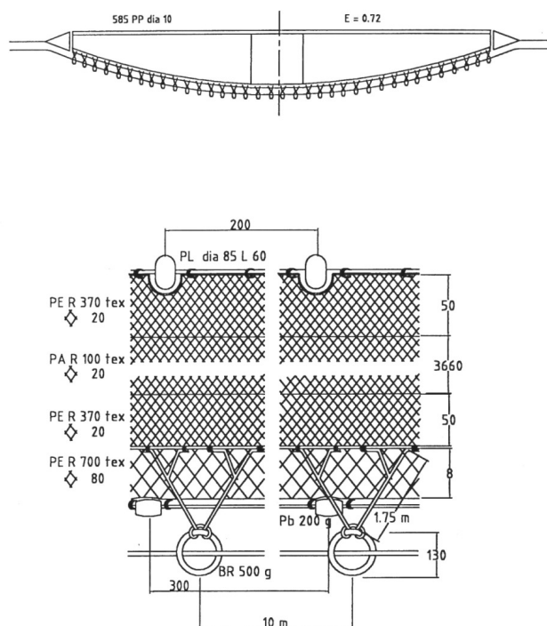
Fig. 2. Details of ring seine design and rigging
