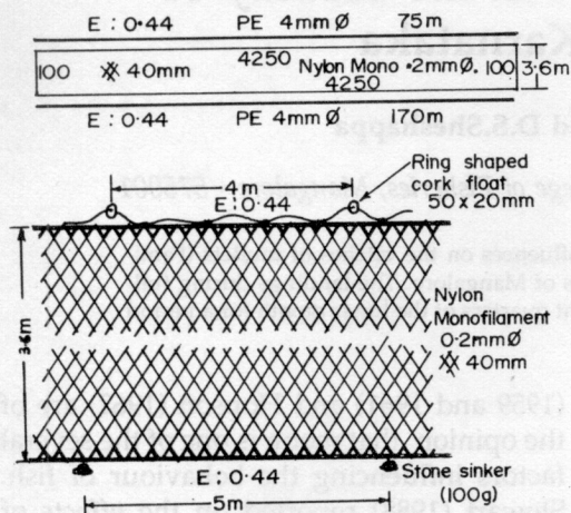
Fig. 1. Details of experimental gill net
