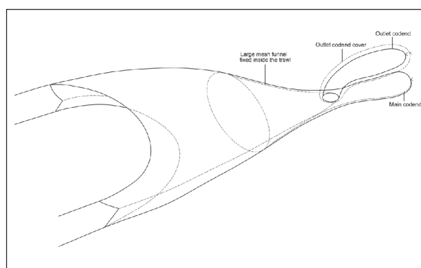
Fig. 2. Perspective view of Sieve net BRD installed in the trawl net
