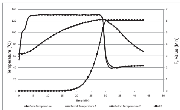
Fig. 3. Heat penetration characteristics and F_0 value of bread spread processed at 130 0 C
