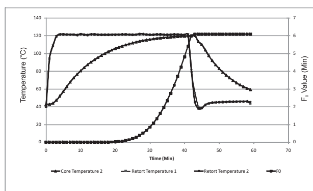
Fig. 2. Heat penetration characteristics and F_0 value of bread spread processed at 121.1 0 C
