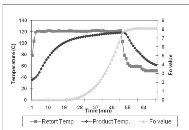
Fig. 1. Heat penetration characteristics and F_0 value of sardine curry in HIPP trays
