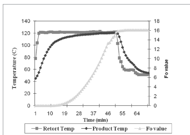
Fig. 2. Heat penetration characteristics and F_0 value of rice in HIPP trays
