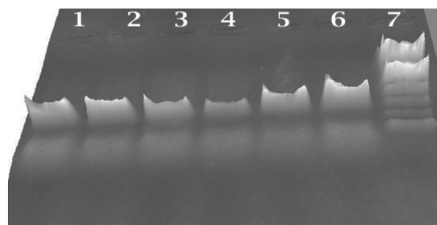
Fig. 2. Salmonella isolates showing the amplification of invA gene (284 bp amplicon) Lane 1 to 5: Salmonella isolates from fish; Lane 6: Salmonella Type culture; Lane 7: 100 bp Marker
