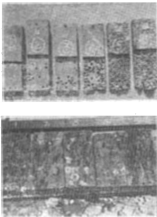
Fig 2 & 3. Pattern of marine borer attack on unprotected wooden test blocks (control) at the C. I. F. T Test Site, Cochin.
