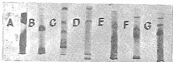
Fig 1. Electrophoretic patterns of muscle myogens of different species of fish and shell fish.
