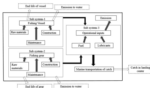
Fig. 2. Block diagram of the studied system. Dotted line represent the system boundary
