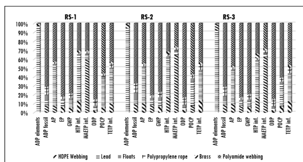
Fig. 5. Relative contribution to environmental impact associated with the subsystem-2 Fishing gear RS-1, RS-2, RS-3
