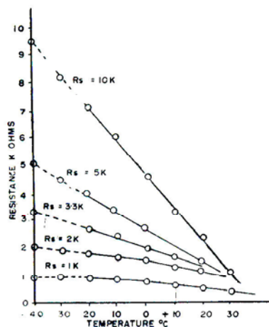
Fig. 2. Linearisation of thermistor with shunt resistance R_s .
