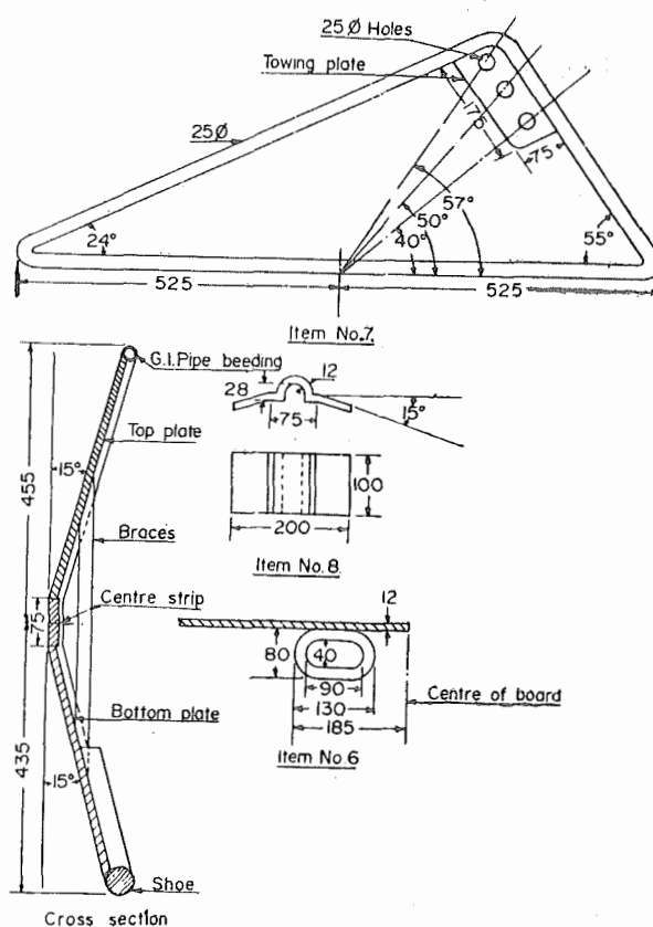
Fig. 2. Details of parts (measurements in mm)
