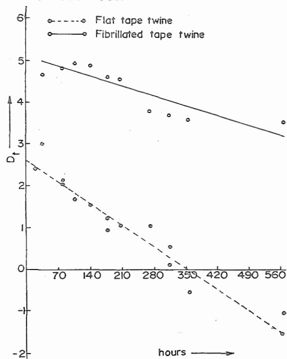
Fig. 2. Plot of the difference between the breaking strengths of the fibrillated tape twine and flat tape twines against the monofilament twines (artificial UV radiation).
