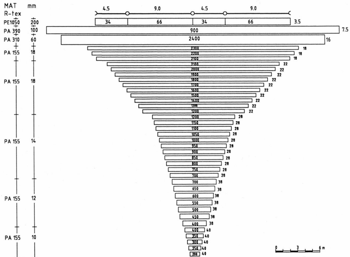
Fig. 1. Design of stake net
