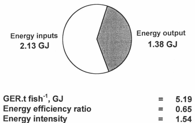
Fig. 3. Results of energy analysis of stake net operations
