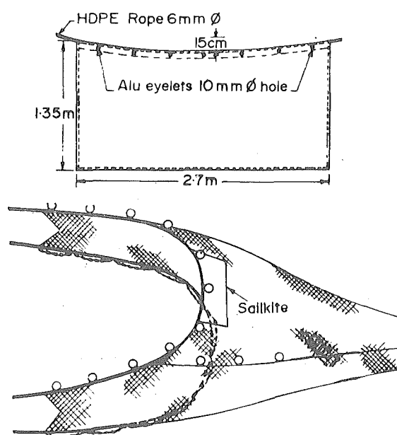
Fig. 1. Construction and method of attachment of sailkite to the trawl.
