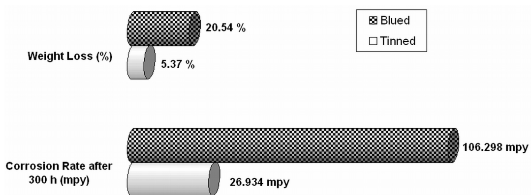
Fig. 2. Performance of fishing hooks after 300 h salt spray exposure
