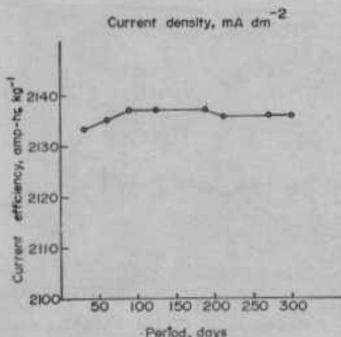
Fig. 6. Plot of anode current efficiency as a function of time at 140 \text{ mA cm}^{-2} .
