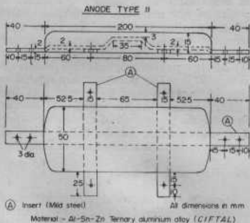
Fig. 2. Anode (Type II) used on steel trawlers
