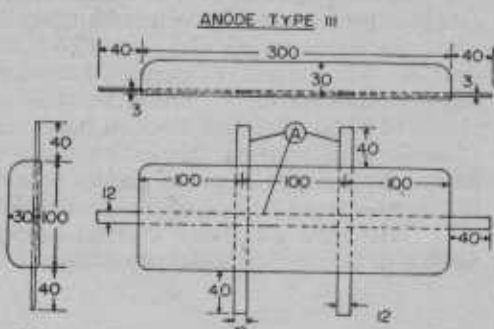
Fig. 3. Large anode (Type III) used on steel trawlers and marine structures
