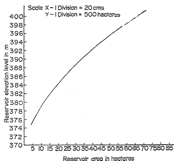
Fig. 4. Hypsographic curve.
