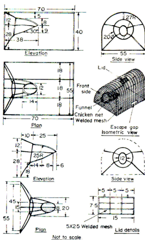
Fig. 1. Design details of modified lobster trap
