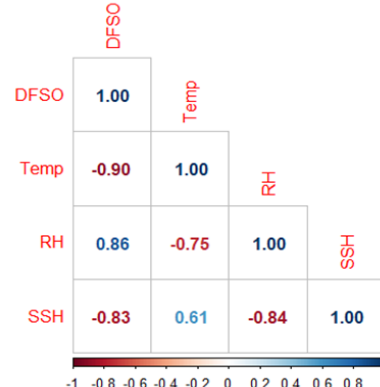
Fig. 2. Correlation between DFSO and climatic factors
