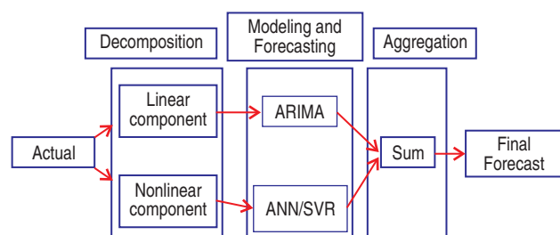
Fig 3 Schematic representation of ARIMA-ANN/SVR hybrid methodology.
