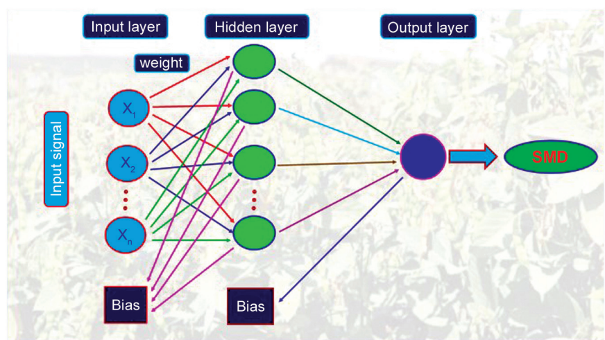
Fig 2 A multilayer perceptron (MLP) architecture with one hidden layer
