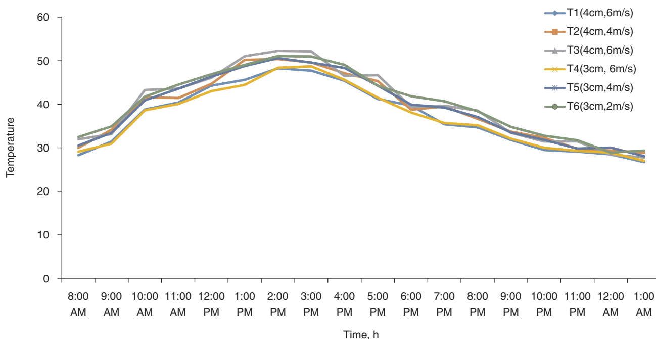
Fig 5 Temperature profiles for various treatment combinations.
