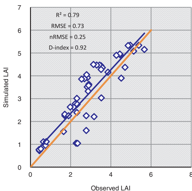
Fig 2 Observed versus InfoCrop-wheat simulated LAI in HD-2967 wheat cultivar under different treatment of sowing date and irrigation levels.
