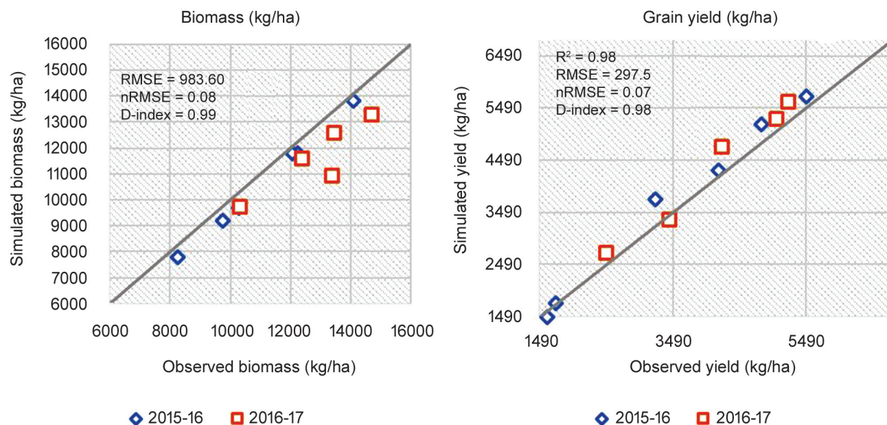
Fig 3 Observed versus InfoCrop-wheat final biomass and grain yield and in HD-2967 wheat cultivar under different treatment of sowing date and irrigation levels.
