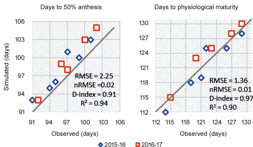
Fig 1 Observed versus InfoCrop-wheat simulated days to 50% anthesis and days to physiological maturity for HD-2967 wheat cultivar under different treatment of sowing date.
