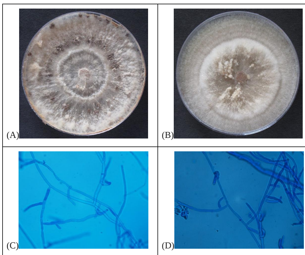
Supplementary Fig 1 Morphology and growth pattern on potato dextrose agar (A) SCRS-2018-1A and (B) SCRS-2018-1B and microscopic images showing mycelia and its branching pattern of two isolates of Rhizoctonia solani in potato dextrose agar (C) SCRS-2018-1A and (D) SCRS-2018-1B.
