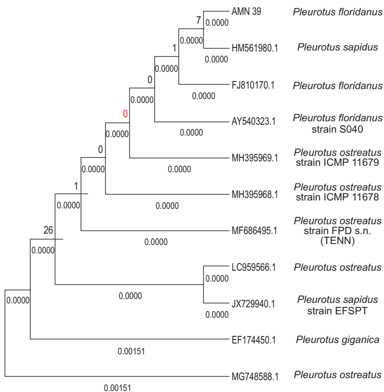
Supplementary Fig. 2 Molecular phylogenetic analysis of AMN 202 ( P. floridanus ) by Maximum Likelihood Method.
