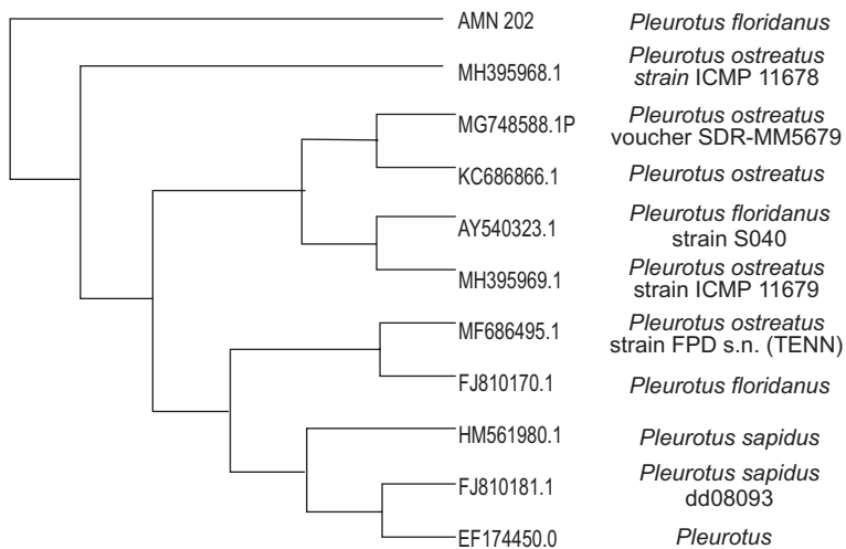
Supplementary Fig. 1 Molecular phylogenetic analysis of AMN 39 ( P. sapidus ) by Maximum Likelihood Method.
