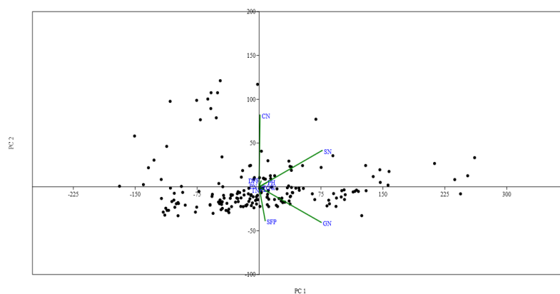
Supplementary Fig 1 Biplot to explain the majority of the data variance using the loading vectors and PC scores.
