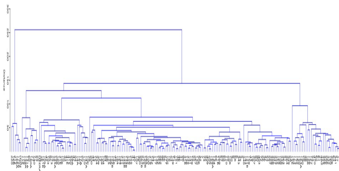
Supplementary Fig 2 Ward method of dendrogram showing genetic relationship among 188 RILs and parents based on phenotypic data.
