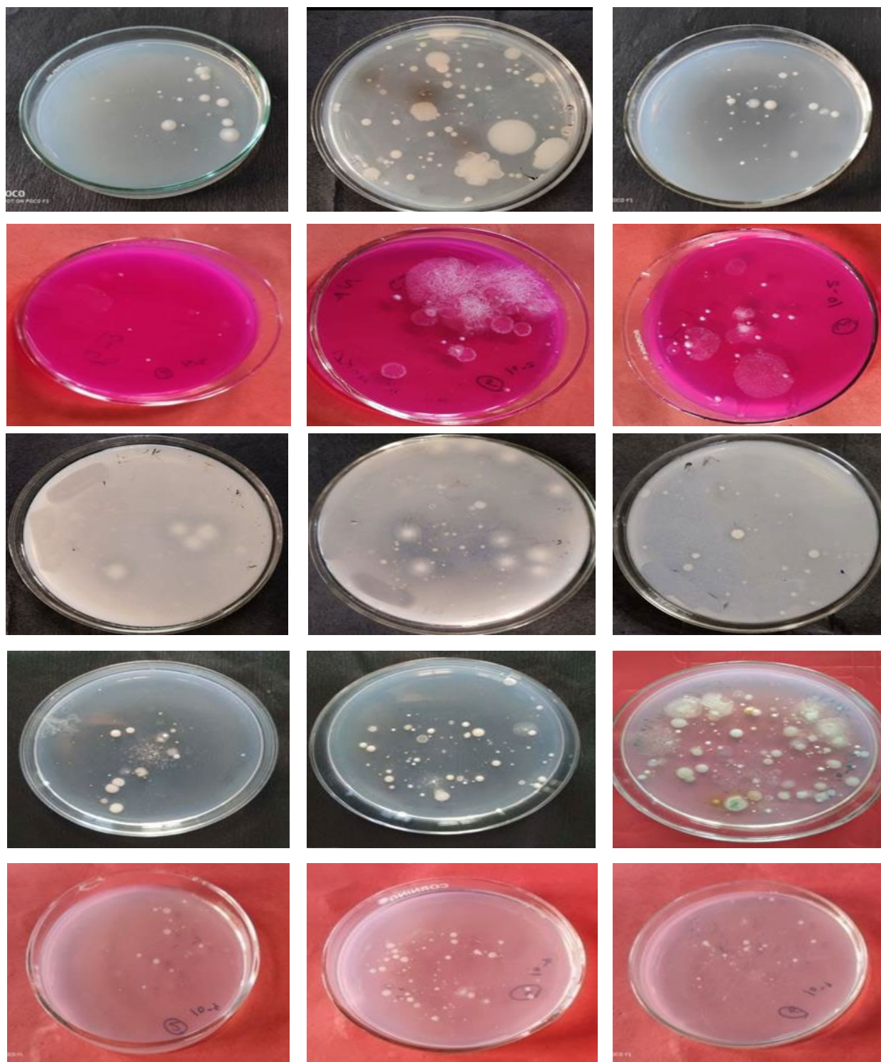
Supplementary Fig. 1 Effect of different nutrient management practices on (a) bacterial (b) fungal (c) PSB (d) actinomycetes (e) Azotobacter population in soil under cotton-wheat cropping system.
