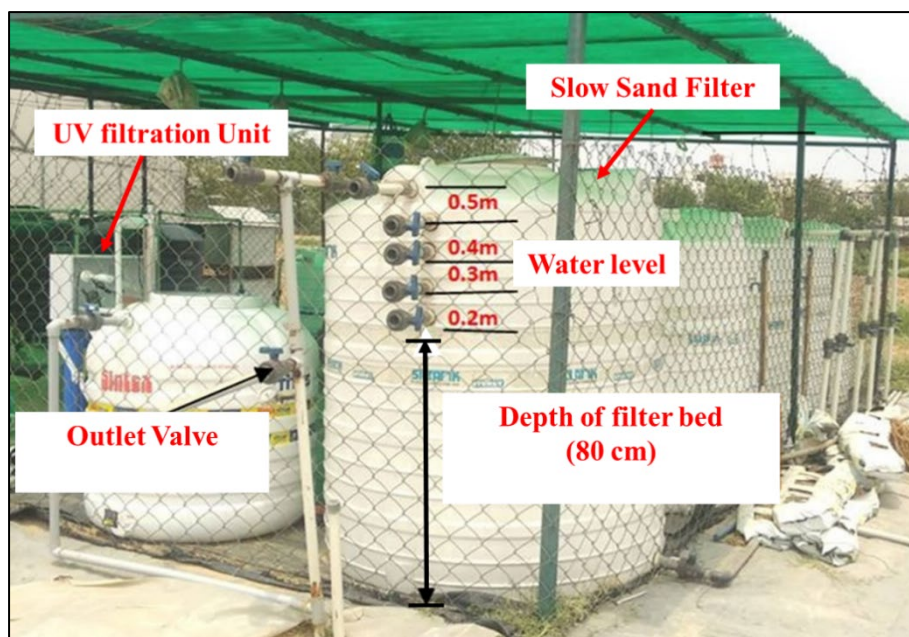
Supplementary Fig. 1 Complete field set-up of slow sand and UV filtration unit.
