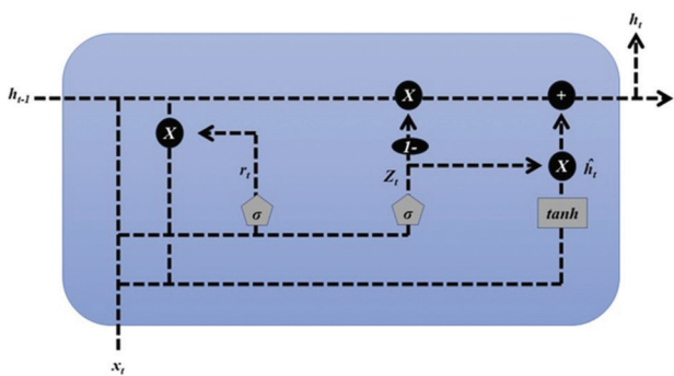
Supplementary Fig. 5 Gated Recurrent Network.
