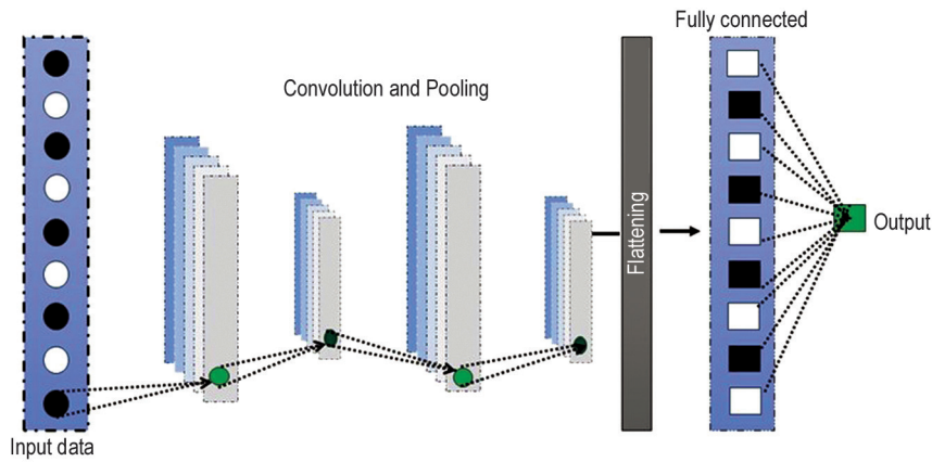
Supplementary Fig. 2 Convolutional Neural Network.
