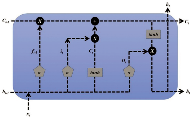
Supplementary Fig. 4 Long Short-Term Memory Network.
