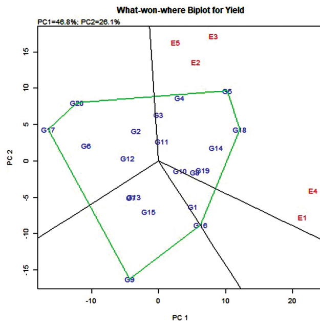
Fig. 3 What-won-where biplot for yield.
