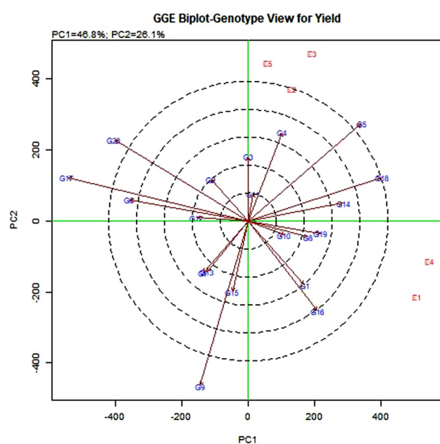
Fig. 2 Genotypic view for seed yield/plant.
