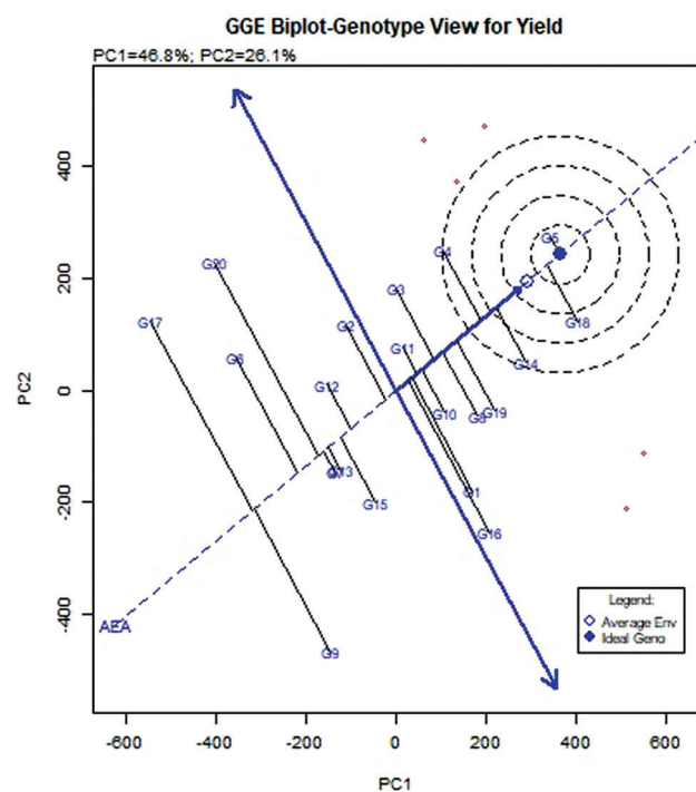
Fig. 1 GGE biplot-genotype view for seed yield.
