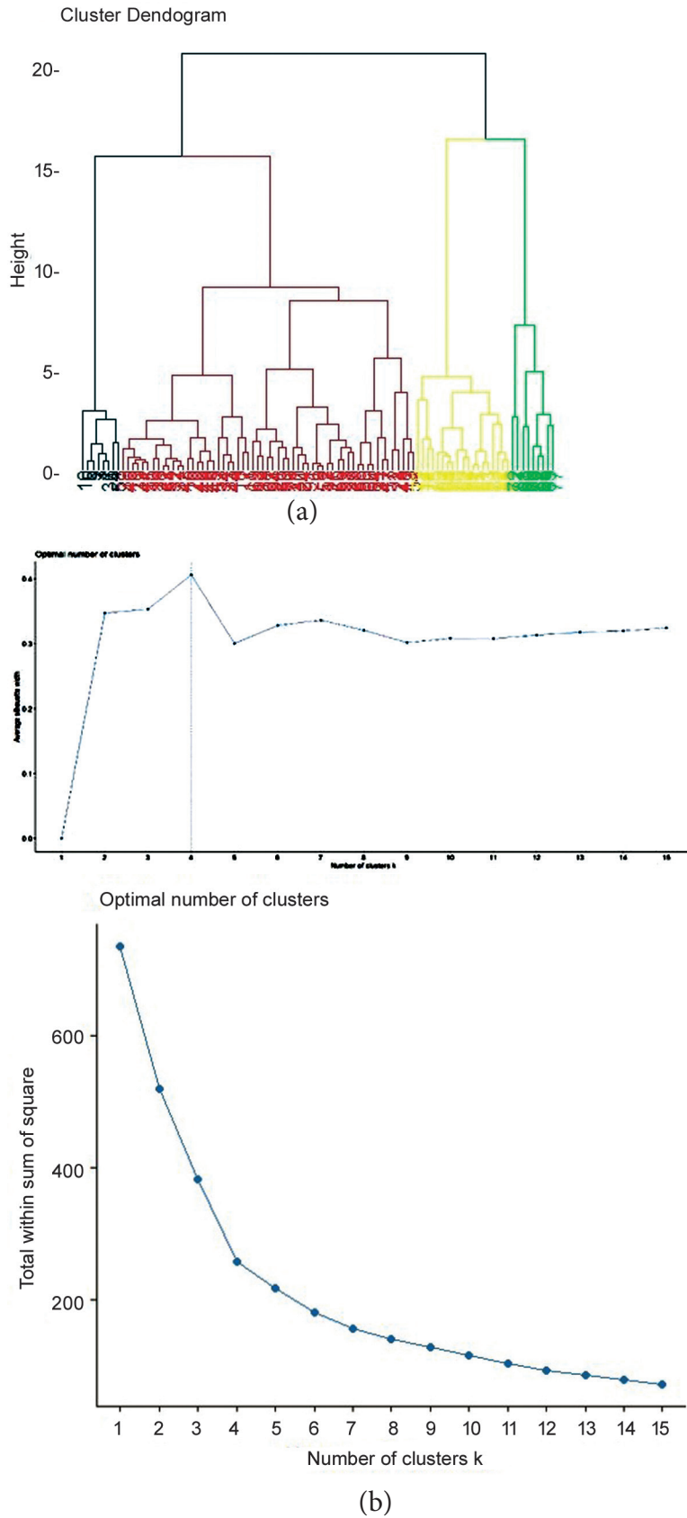
Supplementary Fig. 1 (a) Dendrogram and (b) Scree plot to choose optimal number of clusters.
