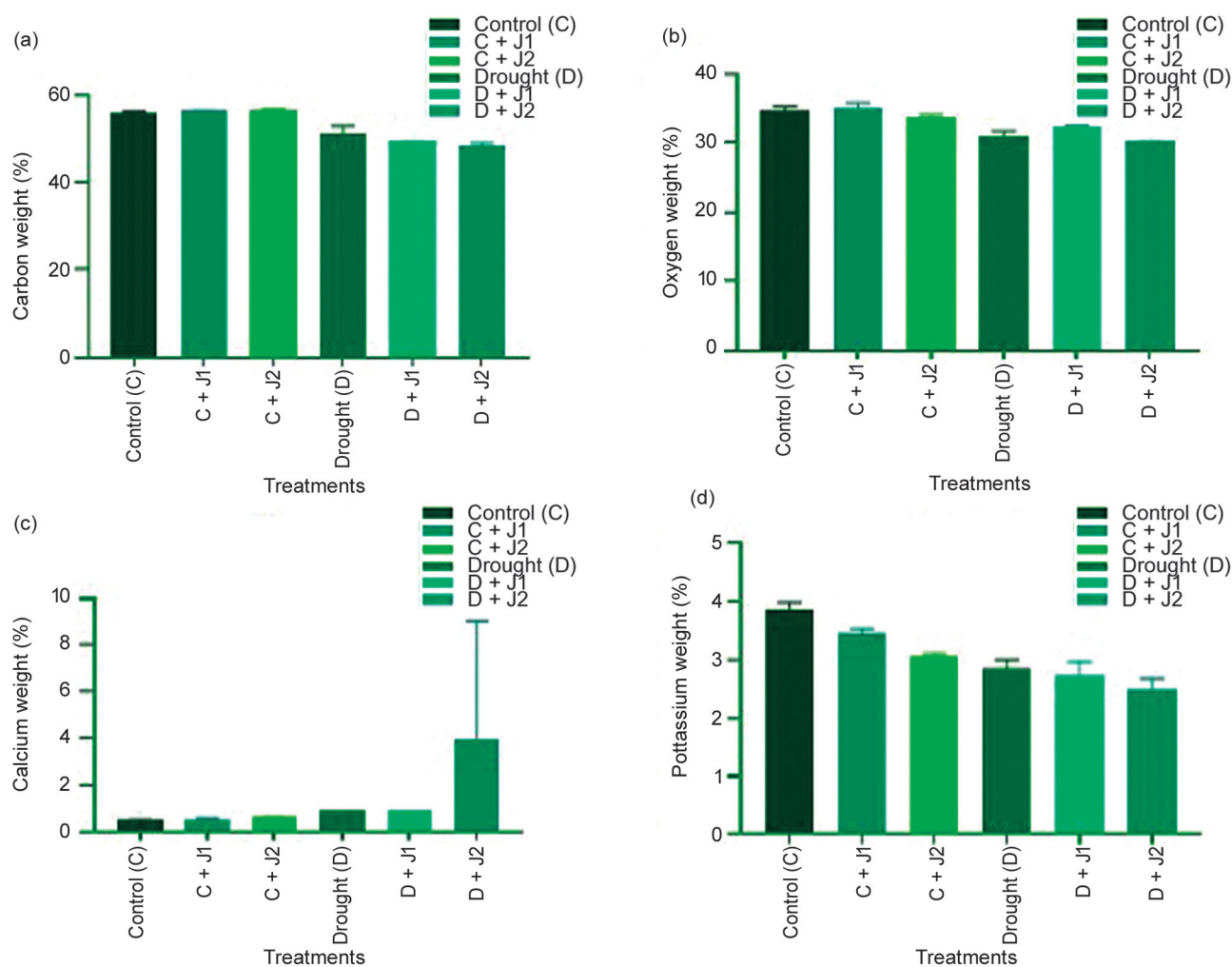
Supplementary Fig. 2 Elemental weight percentages of (a) Carbon weight percentage, (b) Oxygen weight percentage, (c) Calcium weight percentage, and (d) Potassium weight percentage under different treatments.
