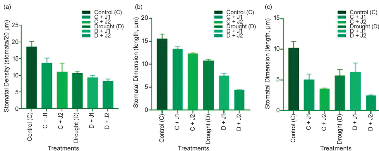
Supplementary Fig. 1 (a) Stomatal density, (b) Stomatal length and (c) Stomatal width under different treatments.
