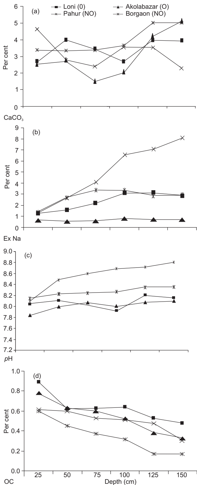
Fig 1 Biophysical sustainability indicators (a) CaCO 3 , (b) exchangeable Na content in organic (Loni and Akolabazar) and non-organic (Pahur and Borgaon) pedons, (c) pH, and (d) organic carbon
