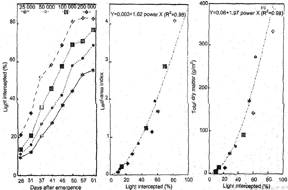
Fig 2 Relationship of leaf-area index (at the time of radiation interception measurement) and per cent photosynthetically active radiation interception measured by ceptometer. Symbols are the same as in Fig 1
